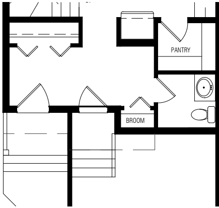
ALTERNATE MAIN FLOOR BATHROOM
